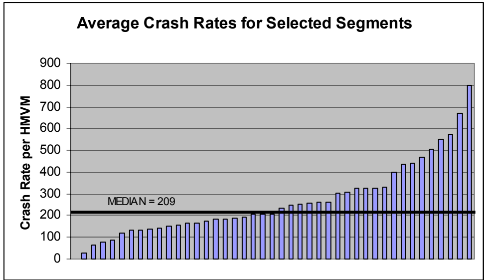
Figure B-3. Average Crash Rates
