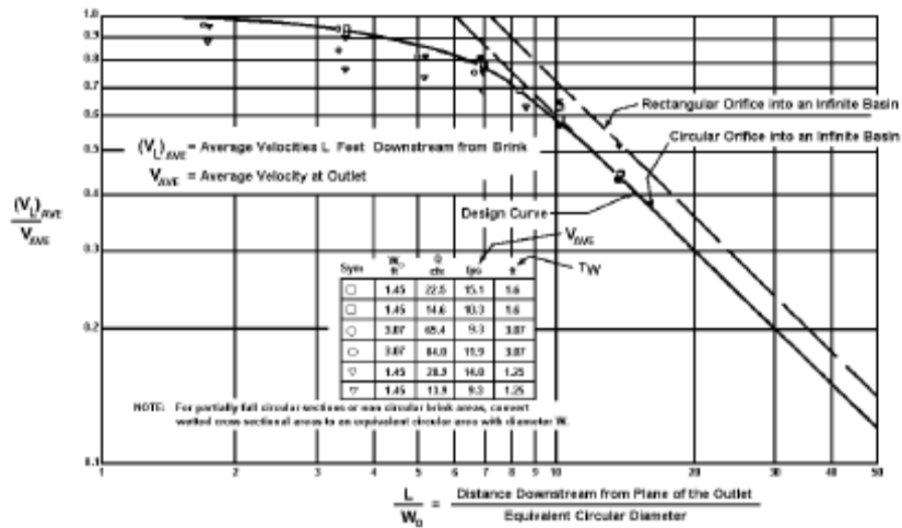
Figure 7-9 Distribution of Centerline Velocity for Flow from Submerged Outlets to Be Used for Predicting Channel Velocities Downstream from Culvert Outlet Where High Tailwater Prevails (Source: USDOT, FHWA, HEC-14, 1983)
