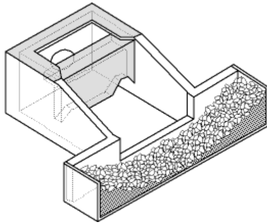
Figure 7-11 Isometric View of Baffled Outlet (Source: Ohio Department of Natural Resources)
