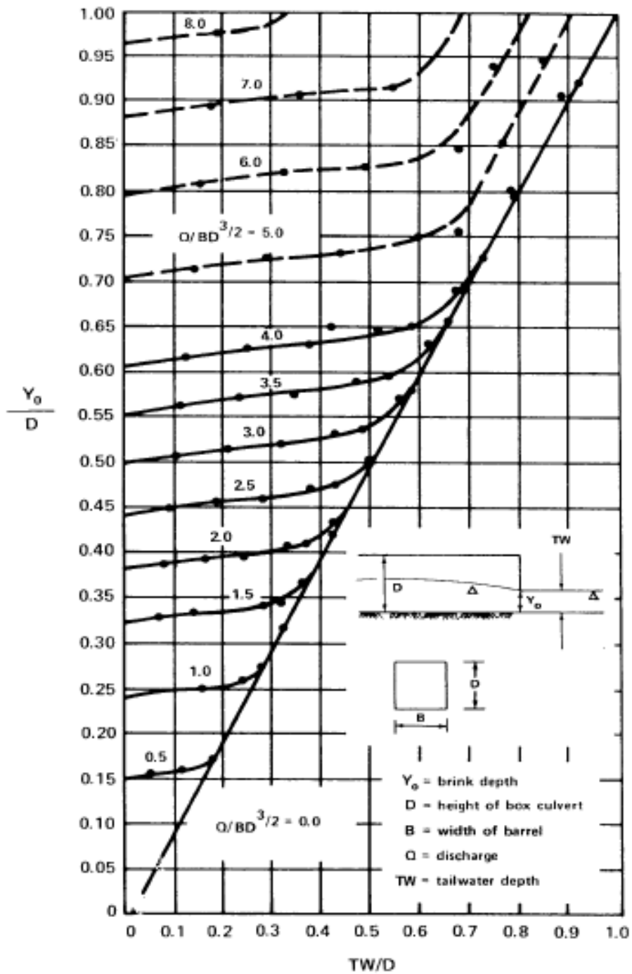
Figure 7-6 Dimensionless Rating Curves for the Outlets of Rectangular Culverts on Horizontal and Mild Slopes (Source: USDOT, FHWA. HEC-14, 1983)
