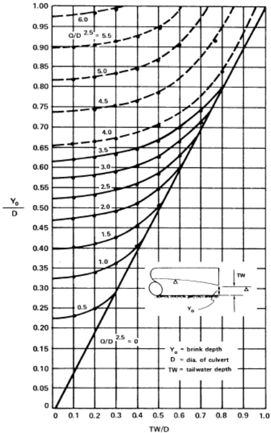
Figure 7-7 Dimensionless Rating Curves for the Outlets of Circular Culverts on Horizontal and Mild Slopes
