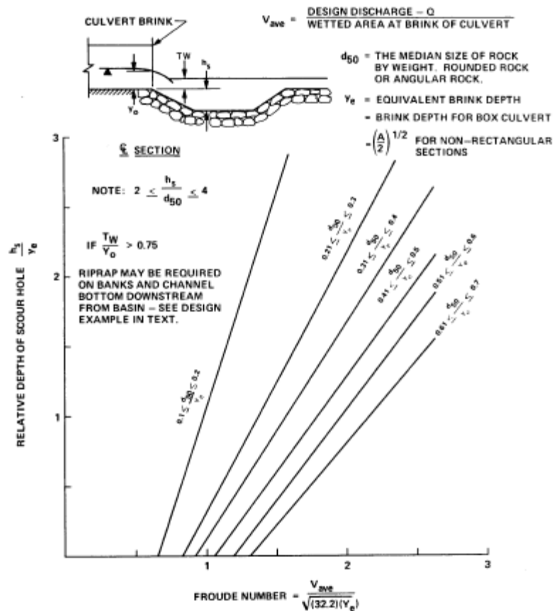
Figure 7-8 Relative Depth of Scour Hole versus Froude Number at Brink of Culvert with Relative Size of Riprap as a Third Variable (Source: USDOT, FHWA, HEC-14, 1983)
