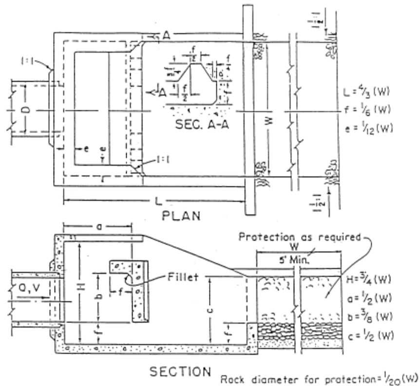
Figure 7-12 Schematic of Baffled Outlet (Source: U.S. Dept. of the Interior, 1978)
