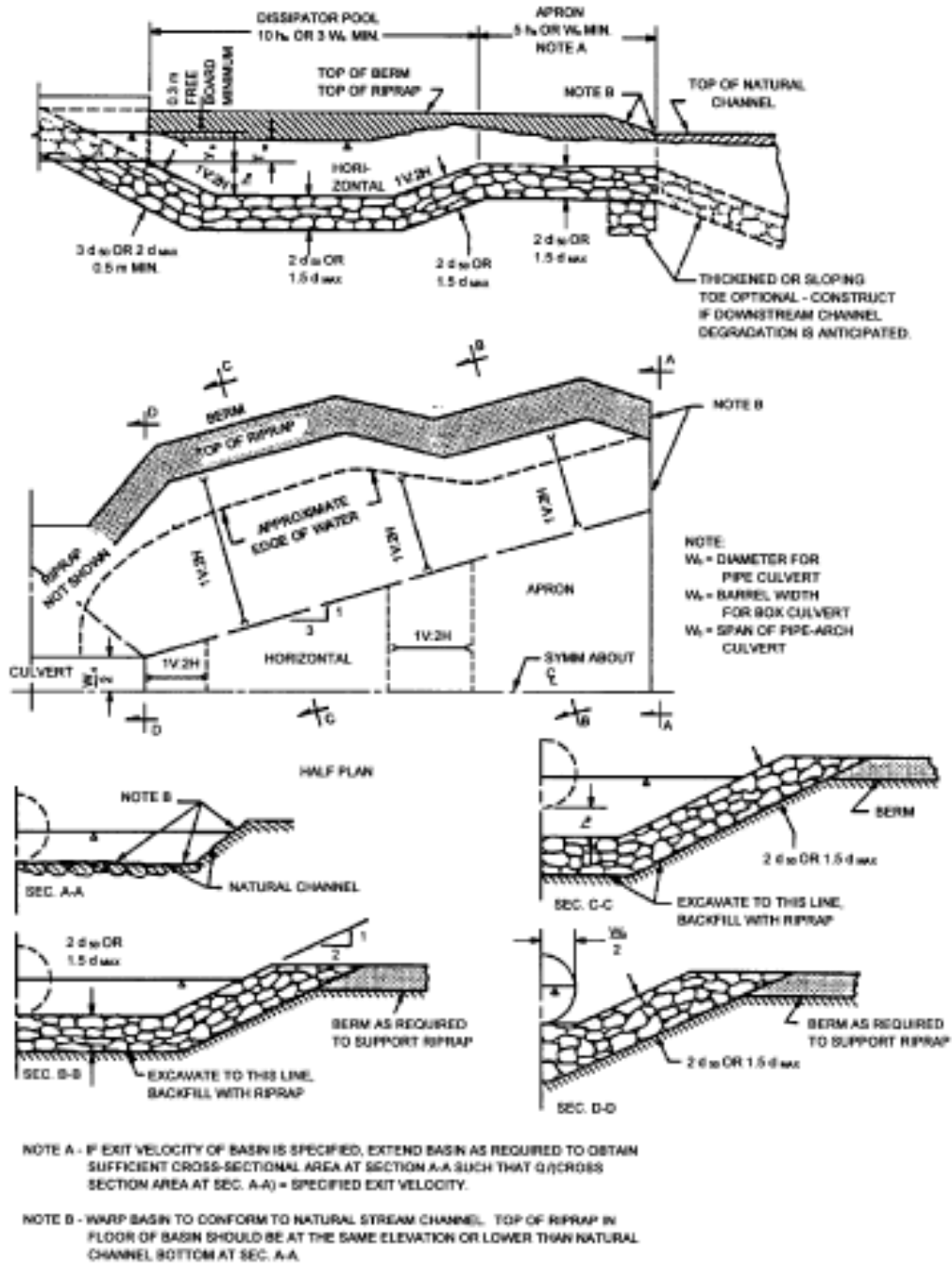
Figure 7-5 Details of Riprap Outlet Basin (Source: Hec-14, 1983)
